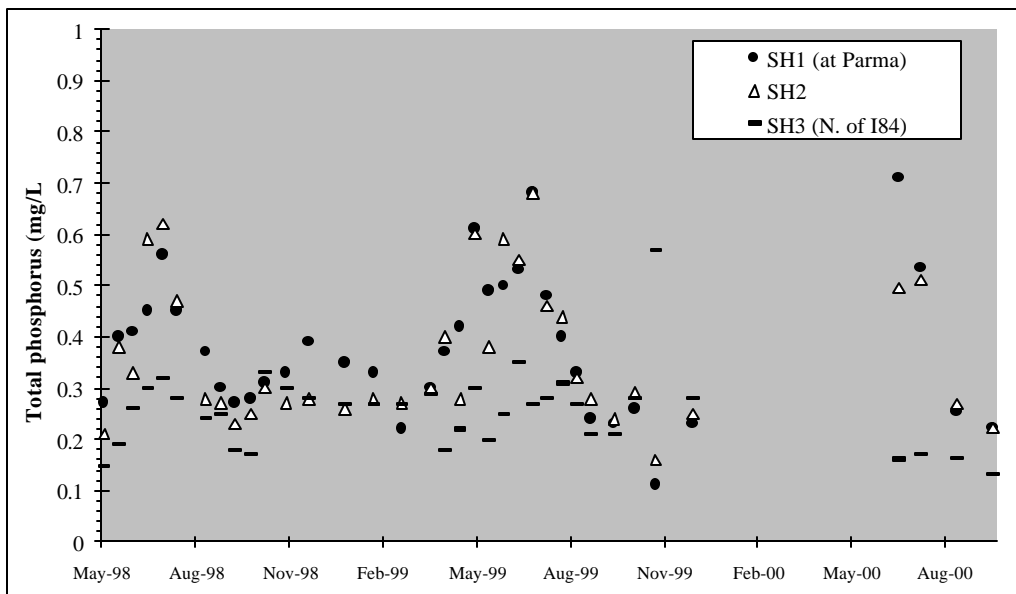
Figure 10. Total phosphorus levels in Sand Hollow Creek, 1998-2000.
